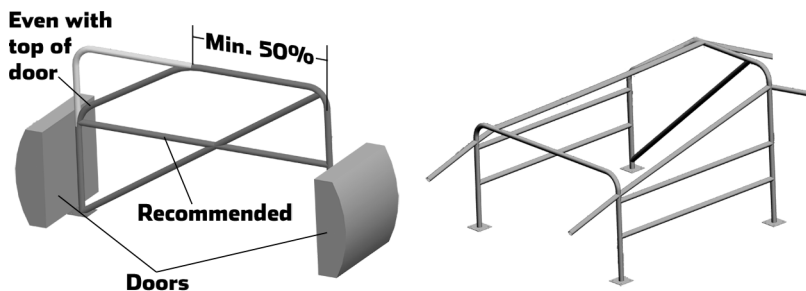
Minimum main hoop - Open Production
