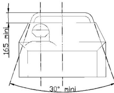
Dessin / Drawing 258A-4
