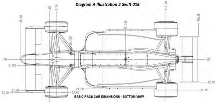
BASIC RACE CAR DIMENSIONS - BOTTOM VIEW
