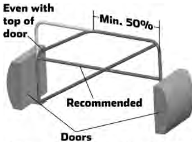
Minimum main hoop - Open Production
