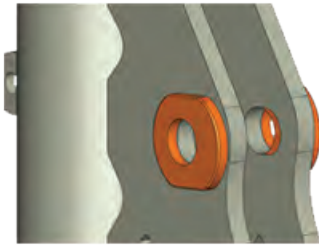
Figure 2: SMG Strut Housing with Camber Slug Installed.
